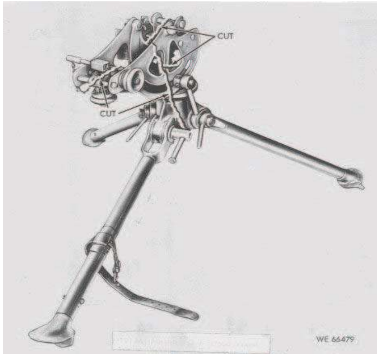
Figure 6. Machine Gun Tripod Mount
